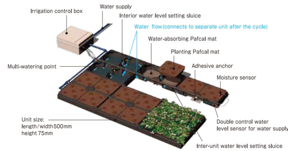
Diagram of the Midori no Yane Light's automatic water supply system (water supplied via level tubes, slight incline tubes, partial reverse incline tubes, and combinations thereof)
